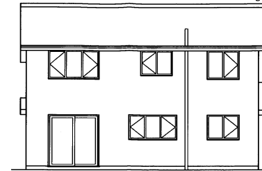
REAR ELEVATION
